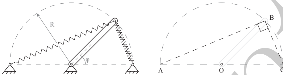
Figure 11: For a spring-to-spring balancer with k_1 = k_2 = k and a_1 = a_2 = r_1 = r_2 = R the constant potential energy can be illustrated elegantly with Thales' theorem: if A , B and C are points on a circle where the line AC is a diameter of the circle, then the angle \angle ABC is a right angle. Using Pythagoras' theorem it is then evident that the total spring energy in the system will be constant for any angle \varphi of the rigid link.
