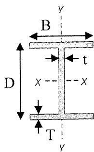
I- Beams
