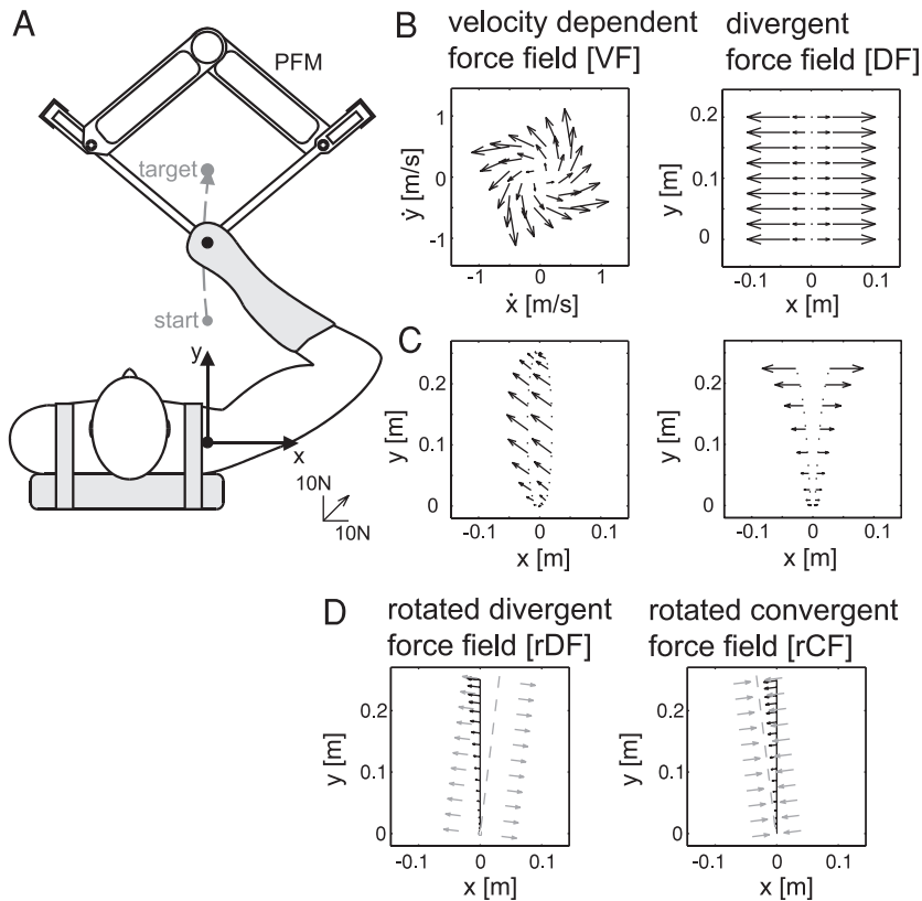
FIG. 2. Experimental setup. A: robotic interface exerts forces on hand during horizontal point-to-point arm movements away from body. B: force in velocity-dependent force field (VF) plotted as function of hand velocity ( left ) and force in divergent force field (DF) plotted as function of hand position ( right ). Vectors indicate direction and magnitude of forces. In VF force vector rotates and increases in magnitude with velocity. In DF force vector increases in magnitude with distance from y -axis. C: force vectors when hand trajectories (dotted curves) are slightly deviated from a straight line along y -axis to left and right . In VF ( left ) applied force vectors are similar despite trajectory variations. DF ( right ) amplifies trajectory variations. D: force in rotated divergent force field (rDF; left ) and rotated convergent force field (rCF; right ). Gray dashed lines and vectors indicate zero force line and direction and magnitude of force at origin of each vector. Black vector denotes applied force when hand trajectories are on straight line connecting start and end targets (black lines). Magnitude and direction of x -force along black lines are identical in rDF and rCF.
